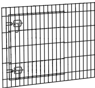
Front Mesh Panel 065.0019 x1
