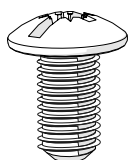
Machine Screw M6x12mm 800.0242 x2
