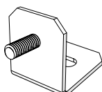
Side Panel to Frame Bracket 064.1022 x4
