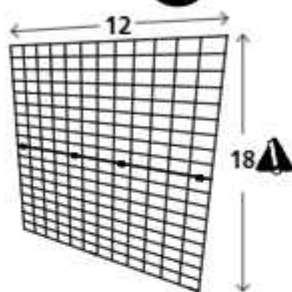
Run Panel Upper Assembly 041.0081 x1
