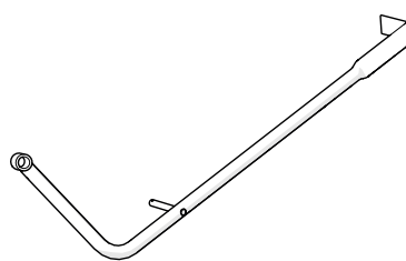
Wheel Arm Left 017.0042 x1
