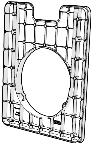
x1 Door Frame Rear 063.1017
