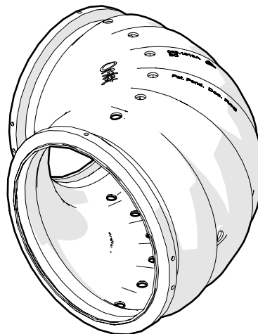
x1 Tunnel 90° 063.1019
